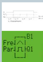
Threshold switch
